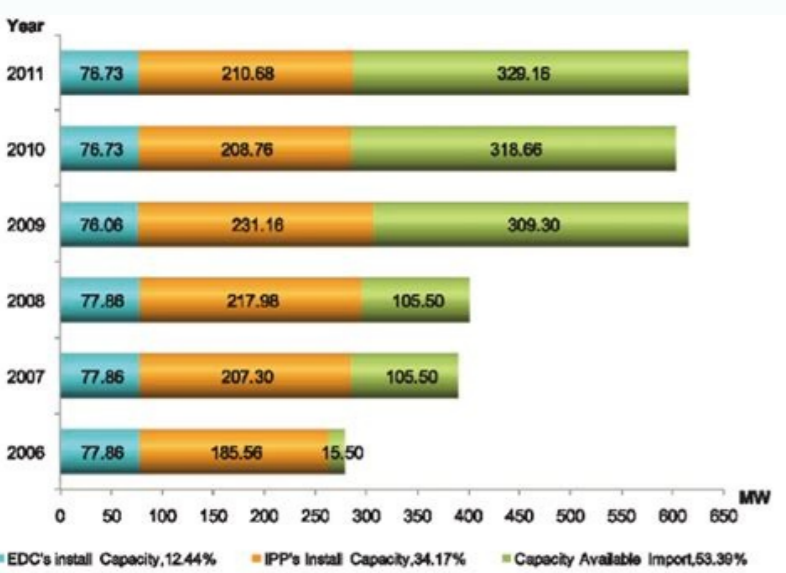
Figure 1: Install Capacity in 2011
